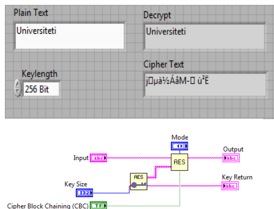
Figure 4. The realization of AES algorithm using LabVIEW
