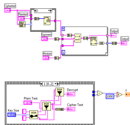
Figure 3. The realization of RSA algorithm using LabVIEW
