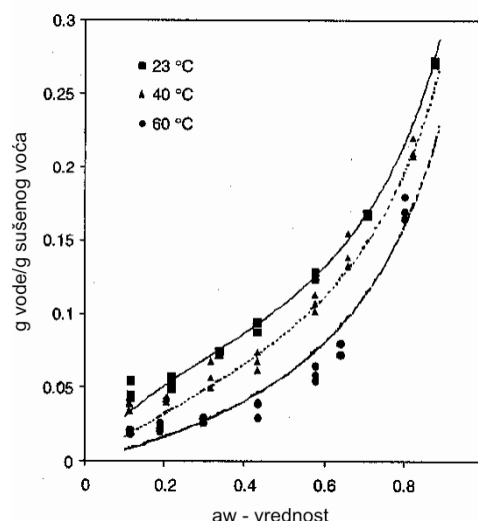
Chart No. 1 Changes aw value of frozen dried fruit to the GAB equation for three different temperatures (Sabani et al., 2004).
